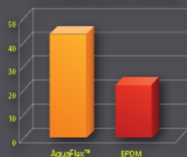
Puncture Resistance (LBS) - ASTM D4833
